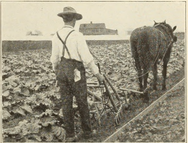
The Planet Jr. Twelve-Tooth Harrow in the Market Garden
